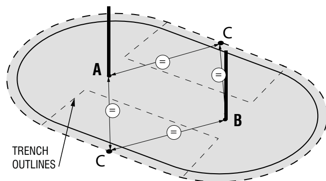
Illustration 2.1 TRENCHES FOR BUTTRESS ASSEMBLIES
