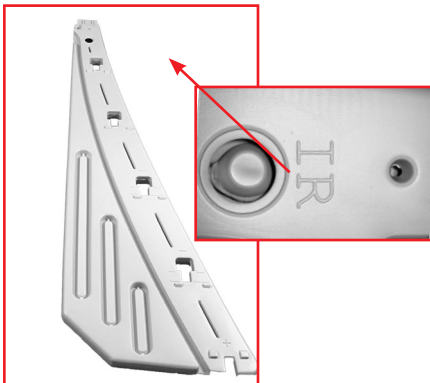
#6: Lay "IR" rail on flat surface.
