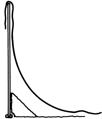
INCORRECT! DO NOT LEAVE A GAP BETWEEN LINER AND COVE. THIS WILL CAUSE DOWNWARD PRESSURE ON THE LINER. CORRECT THIS CONDITION IF IT OCCURS.
